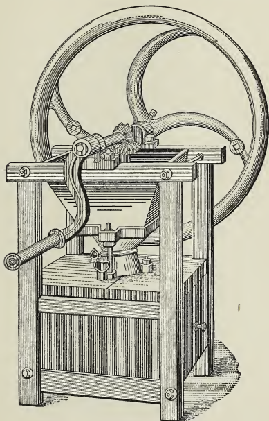
FIG. 1.—Mill for Grinding Resins.
